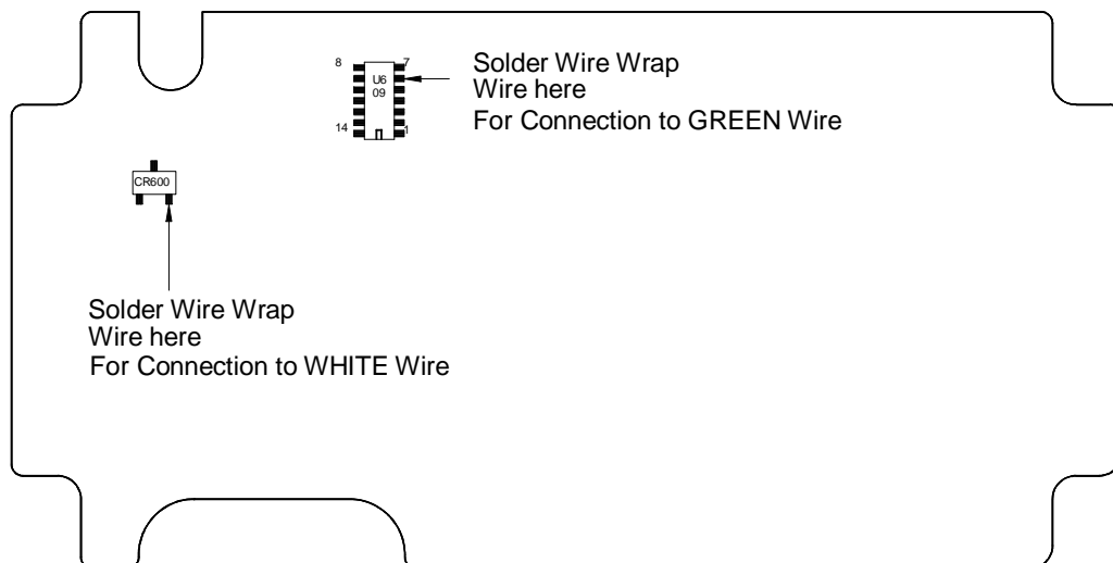
EFJ VIKING GT Audio/Logic Board BOTTOM VIEW
