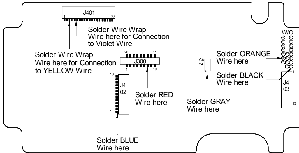
EFJ VIKING GT Audio/Logic Board TOP VIEW
